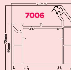
Large Sidelight Frame
