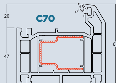
Chamfered Door/Sidelight Frame
