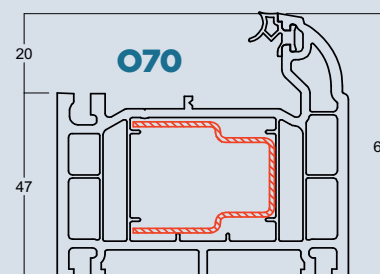
Ovolo Door/Sidelight Frame
