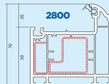
Ovolo Door/Sidelight Frame
