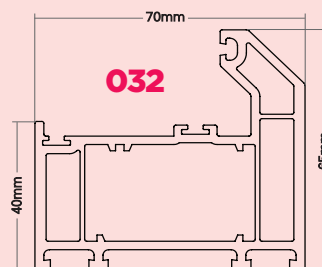
Small Composite Door Frame
