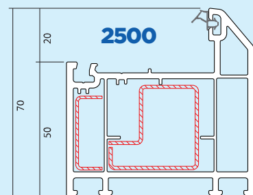
Chamfered Door/Sidelight Frame
