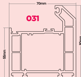
Large Composite Door Frame
