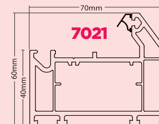
Small Sidelight Frame
